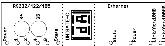
Picture 3: Front panel: Rotary switches and LEDs (only hard.-rev. A)
