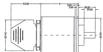
ROTARNOCK RS232 or RS485, version IP54
