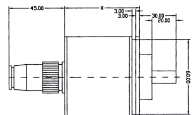
ROTARNOCK 100 with integrated PROFIBUS protection class IP65 and ROTARNOCK 100 with integrated Fieldbus protection class IP65
